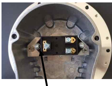
Adjusting screw for calibrating switching point
